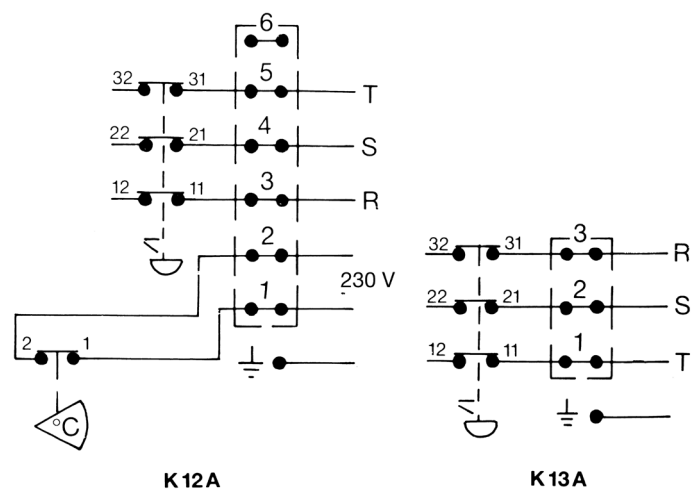
Wiring diagram
